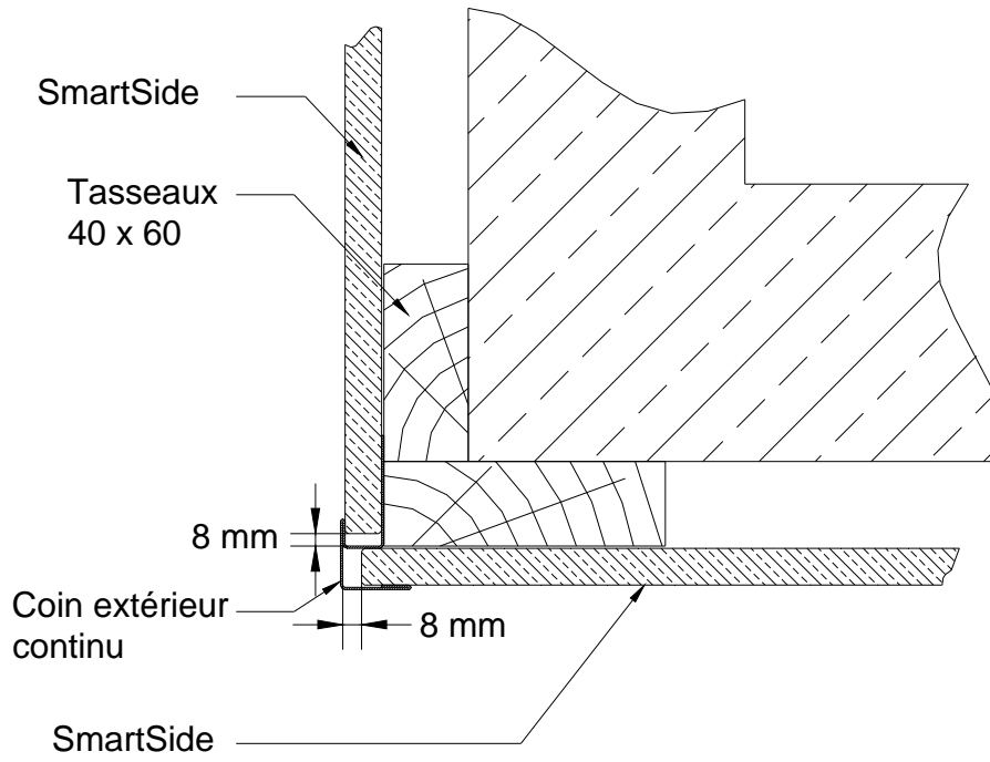
Figure 7 – Angle sortant
