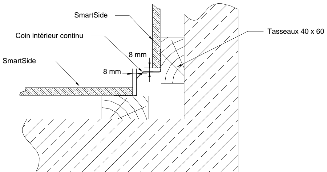
Figure 8 – Angle rentrant
