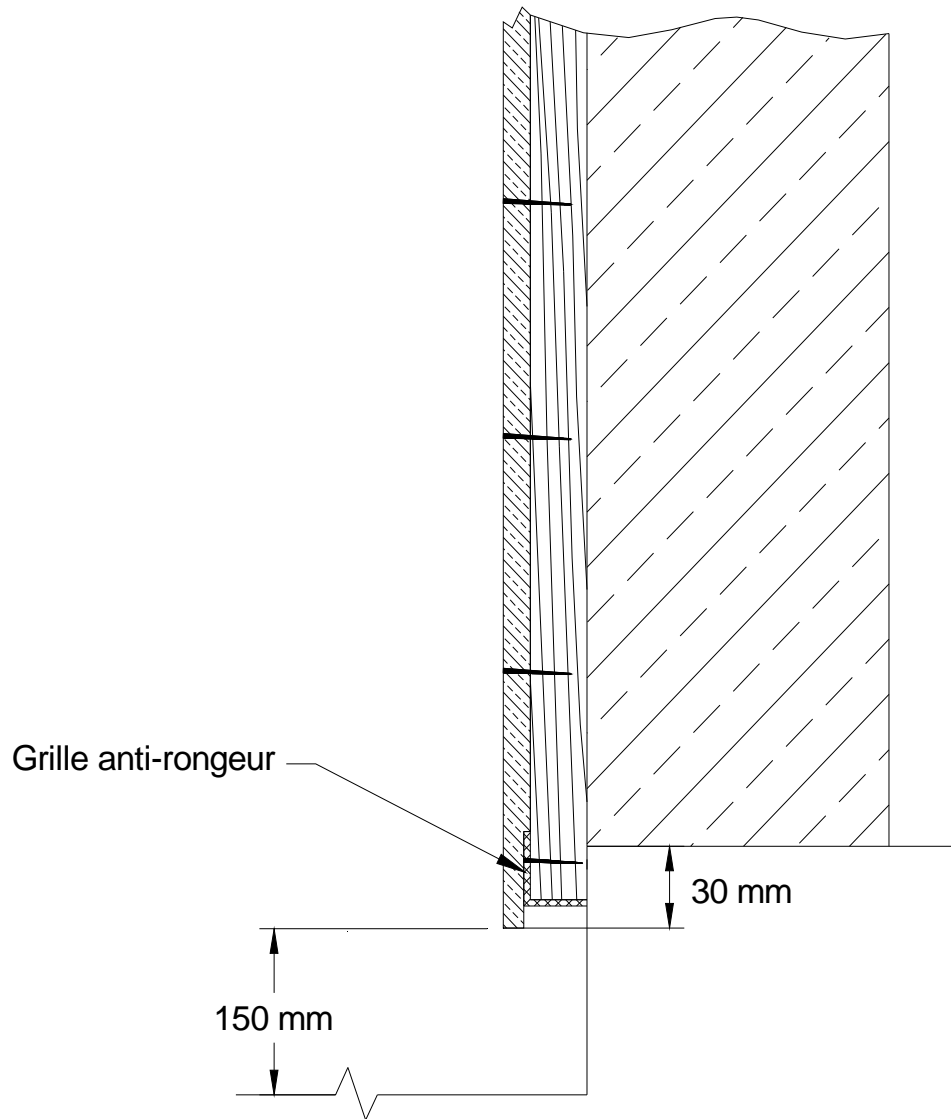
Figure 17 – Grille anti-rongeur
