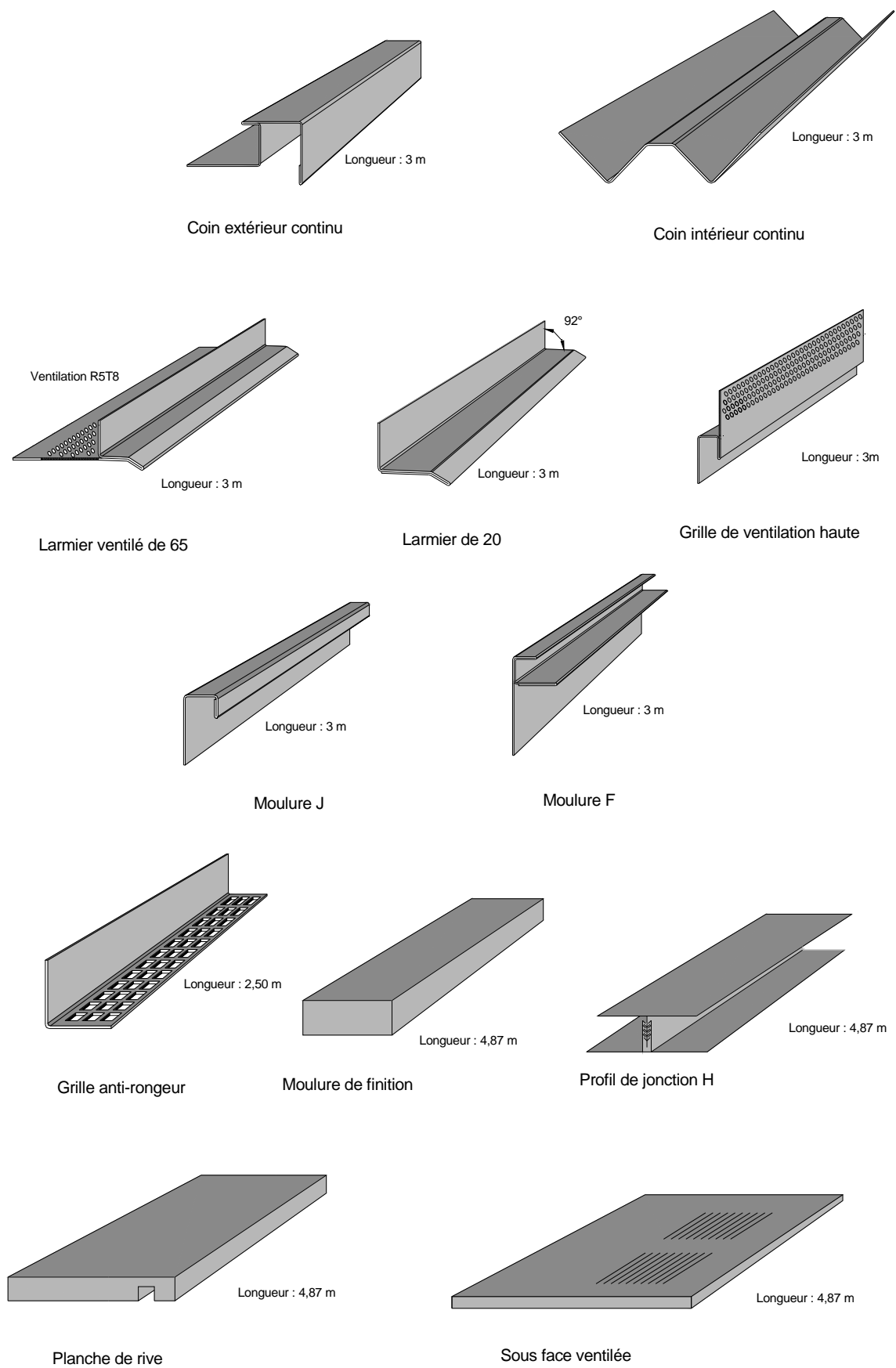
Figure 2 – Accessoires des panneaux SmartSide
