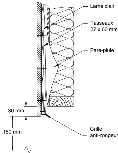
Figure 3 – Pose verticale Panneaux
