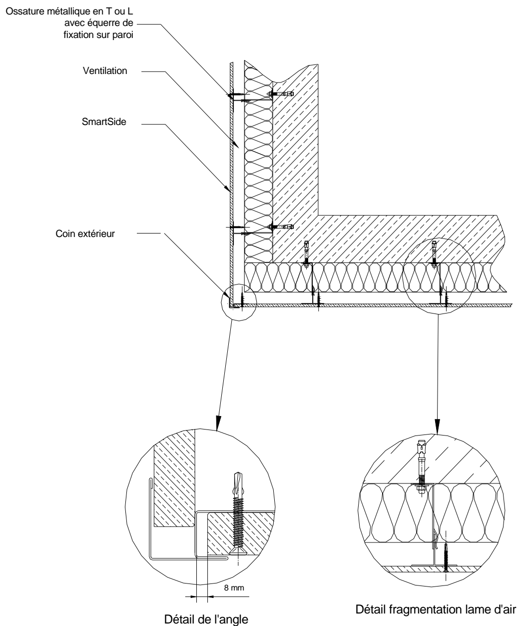
Figure 23 – Angle sortant
